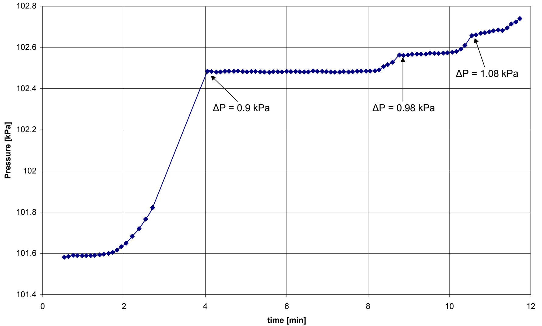
Bubble-Point test of a coffee filter at T = 25 °C, Liquid - isopropanol 91%, (10mm height)
